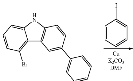
Intermediate B
