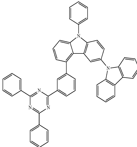
Compound 96
