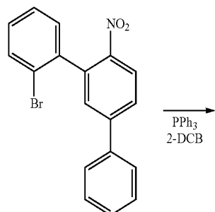
Intermediate A
