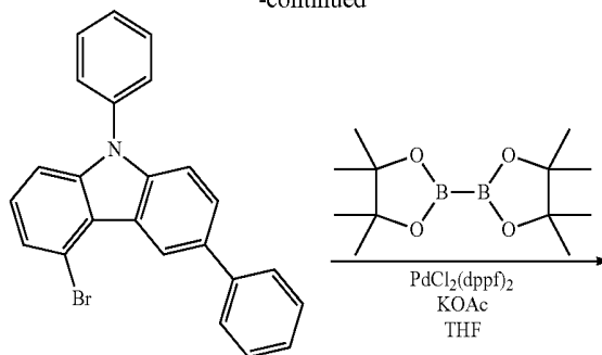
Intermediate C
