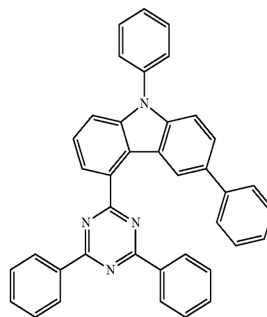
Compound 1
