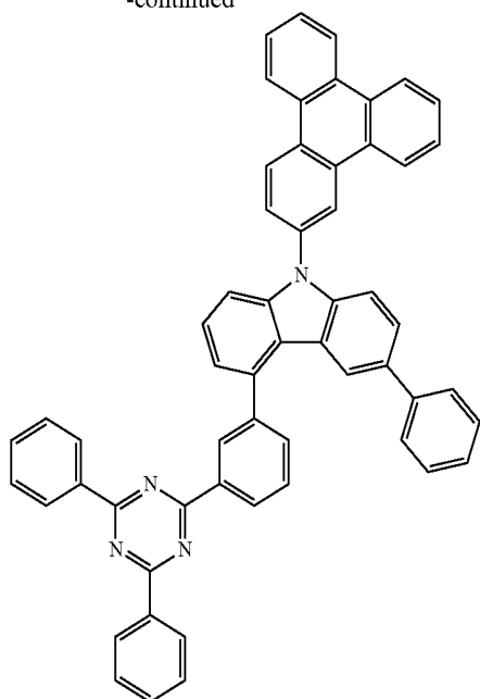
Compound 36
