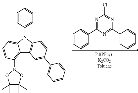
Intermediate D
