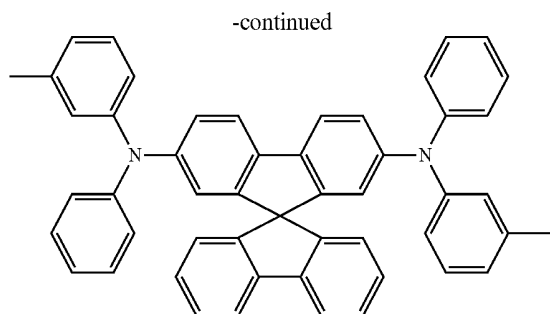
Spiro-TPD
