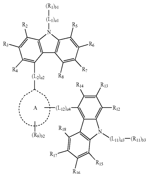
Formula 1B
