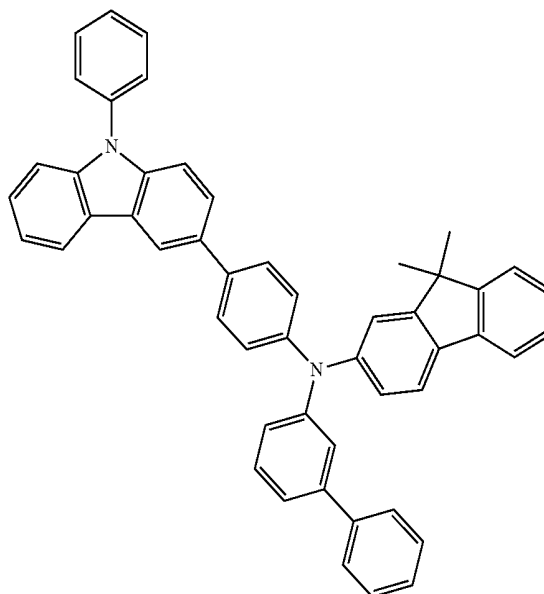
Formula 201A
