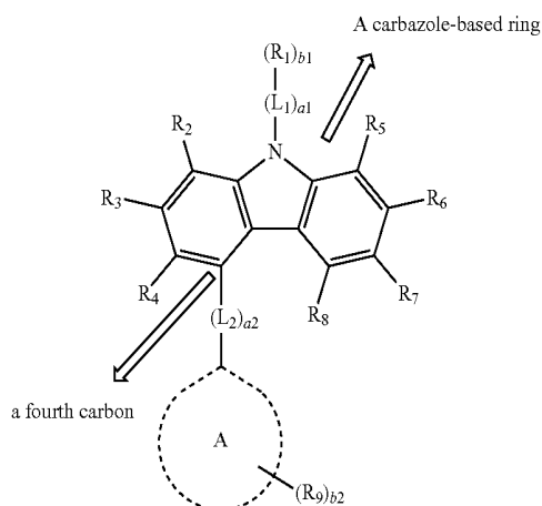
Formula 1A’
