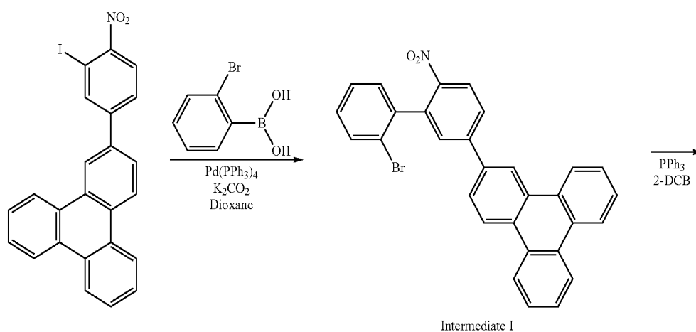
Intermediate I
