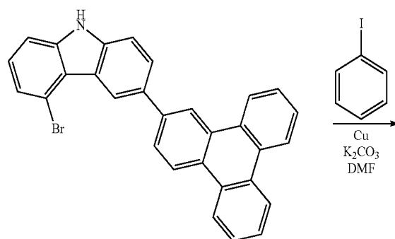
Intermediate J
